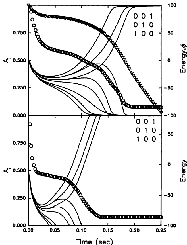
FIG. 1. Plot of the nine A_i concentrations (lines) for the chemical neural network given by Eqs. 1 and 15 ( Upper ) and the reduction of that network to a Hopfield network given by Eqs. 4 and 14 ( Lower ). Both networks start with identical initial conditions and both decay to the same final state (denoted by the matrix of neuron activity in the upper right-hand corners). The energy function (Eq. 5) is indicated by circles, and in Upper \phi (Eq. 23) is indicated by triangles.
