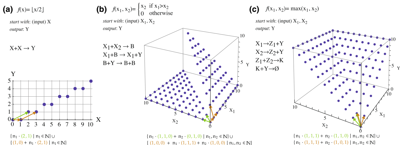
Fig. 1 Examples of deterministically computable functions. (Top) Three functions and examples of CRNs deterministically computing them. The input is represented in the molecular count of X (for a ), and molecular counts of X_1, X_2 (for b and c ). The output is represented by the molecular count of Y . Example a computes via the relative stoichiometry of reactants and products of a single reaction. In example b , the second and third reactions convert B to Y and vice versa, catalyzed by X_1 and B , respectively. Thus, if there are any X_1 remaining after the first reaction finishes (and thus x_1 > x_2 ), all of B can get converted to Y permanently (since some B is required to convert Y back to B ). Since in this case the first reaction produces x_2 molecules of B , x_2 molecules of the output Y are eventually produced.
