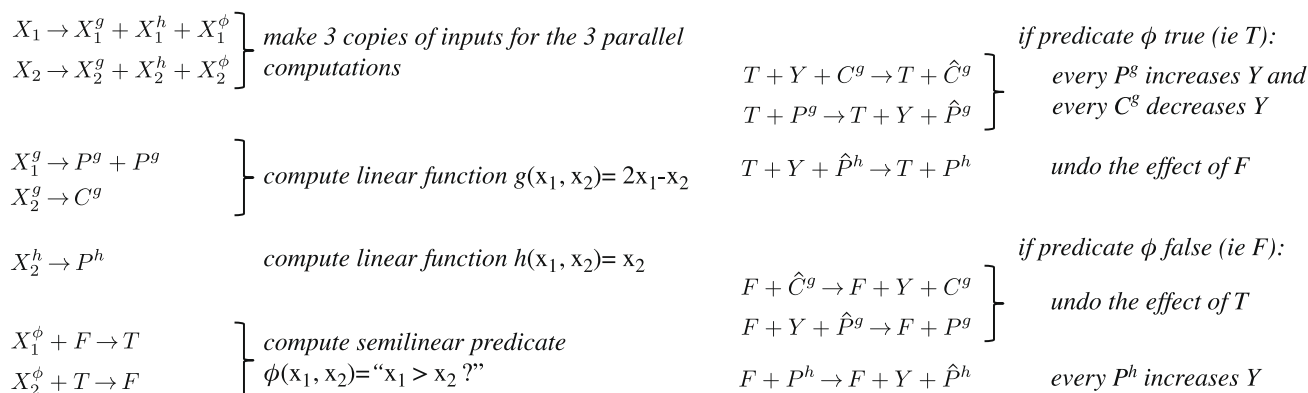
Fig. 2 An example capturing the essential elements of our systematic construction for computing semilinear functions (Lemma 4.4). To compute the target semilinear function, we recast it as a piecewise function defined in terms of linear functions, such that semilinear predicates can decide which of the linear functions is applicable for a given input (this recasting is possible by Lemma 4.3). a The graph of the target function visualizing the decomposition into linear functions. b A CRN deterministically computing the target function with intuitive explanations of the reactions. We use tri-molecular reactions for simplicity of exposition; however, these can be converted into a sequence of bimolecular reactions. Note that we allow an “initial context”: a fixed set of molecules that are always present in the initial state in addition to the input. The linear functions g and h are computed monotonically by representing the output as the difference of P (“produce”) minus C (“consume”) species. Thus although
